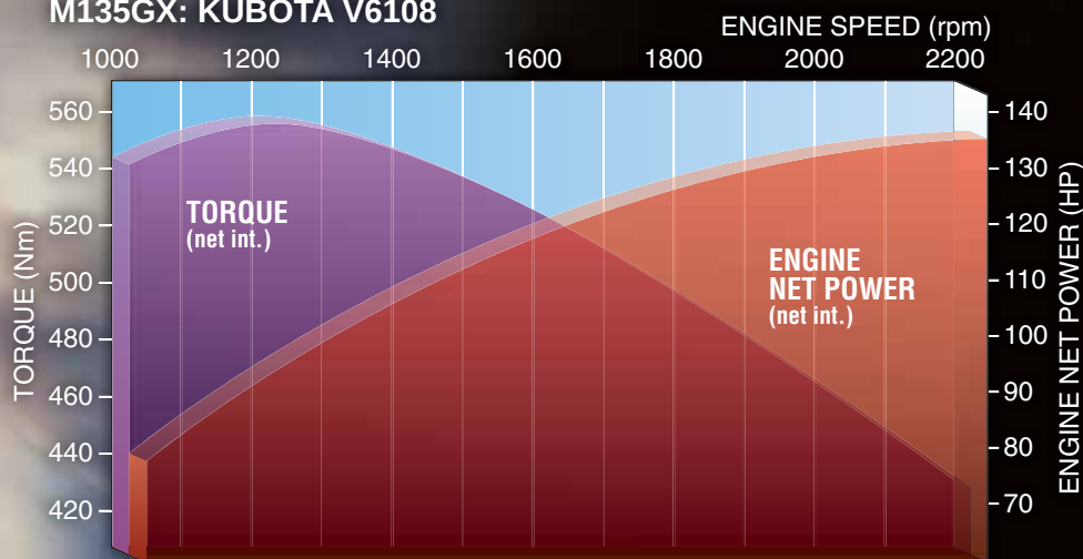
M135GX: KUBOTA V6108
